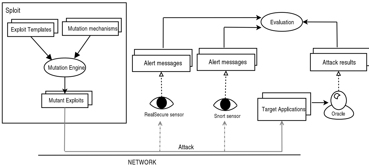
Figure 3: Exploit mutation framework.
