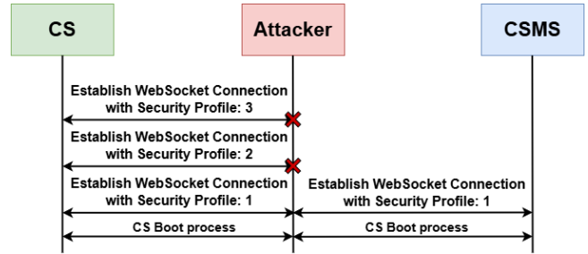
Figure 4: M4 SP3 or SP2 downgrade to SP1 MitM attack.
