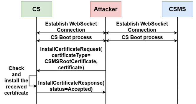
Figure 2: M2 MitM SP2 via malicious CSMS certificate upgrade.
