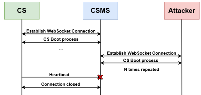
Figure 6: CSMS DoS Attack (D1).
